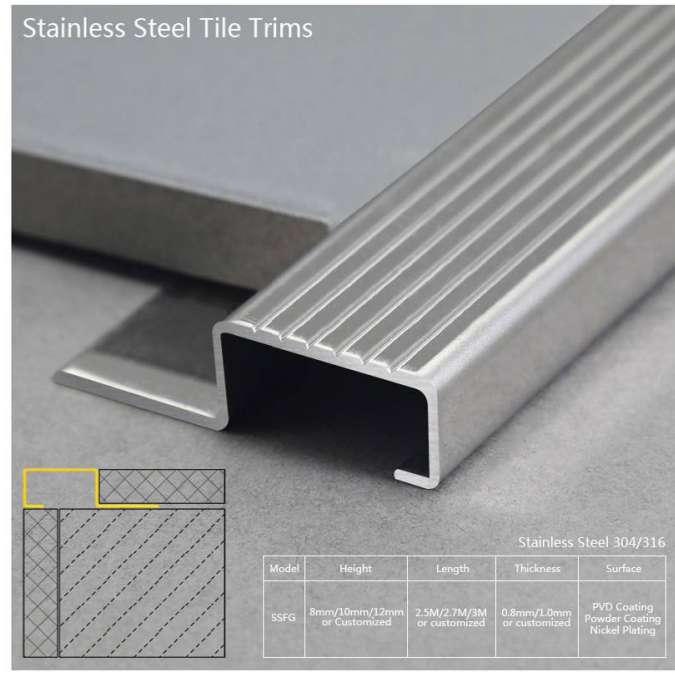
Size Details Specification Can be Customized
