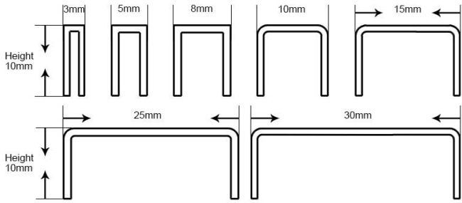
Stainless Steel Tile Trims
