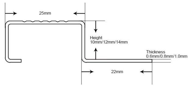
Size Details Specification Can be Customized
