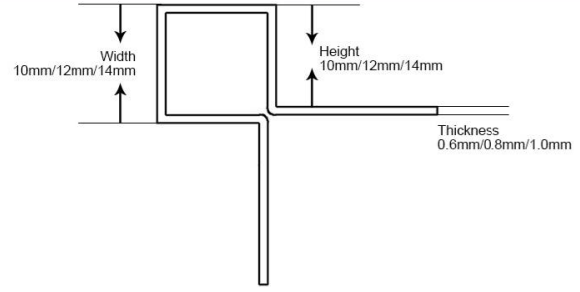
Size Details Specification Can be Customized
